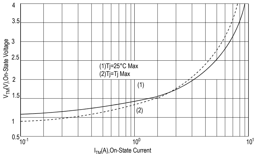
FIG.5: On-state characteristics(Max)
